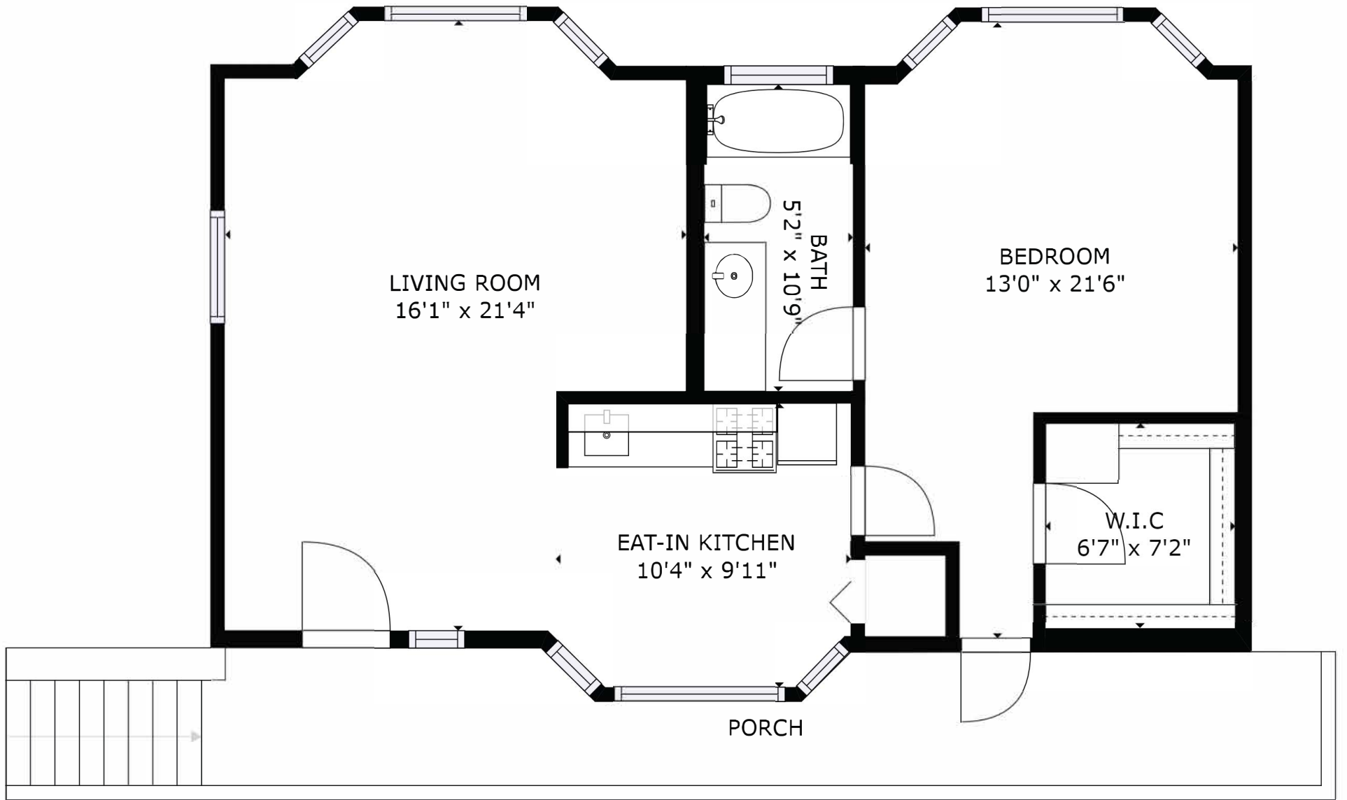
FLOOR 1
